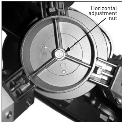
Fig. 6: Horizontal adjustment nut. (View of the underside of the base.)
